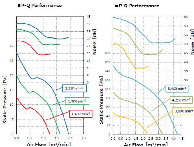
Low-speed Model High-speed Model Air volume & static pressure standard properties (rated voltage)
